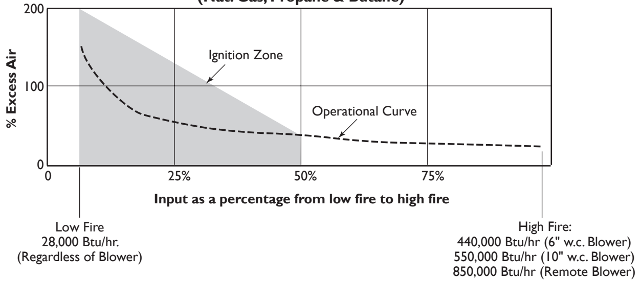
Typical Operational Curve & Ignition Zone (Nat. Gas, Propane & Butane)
